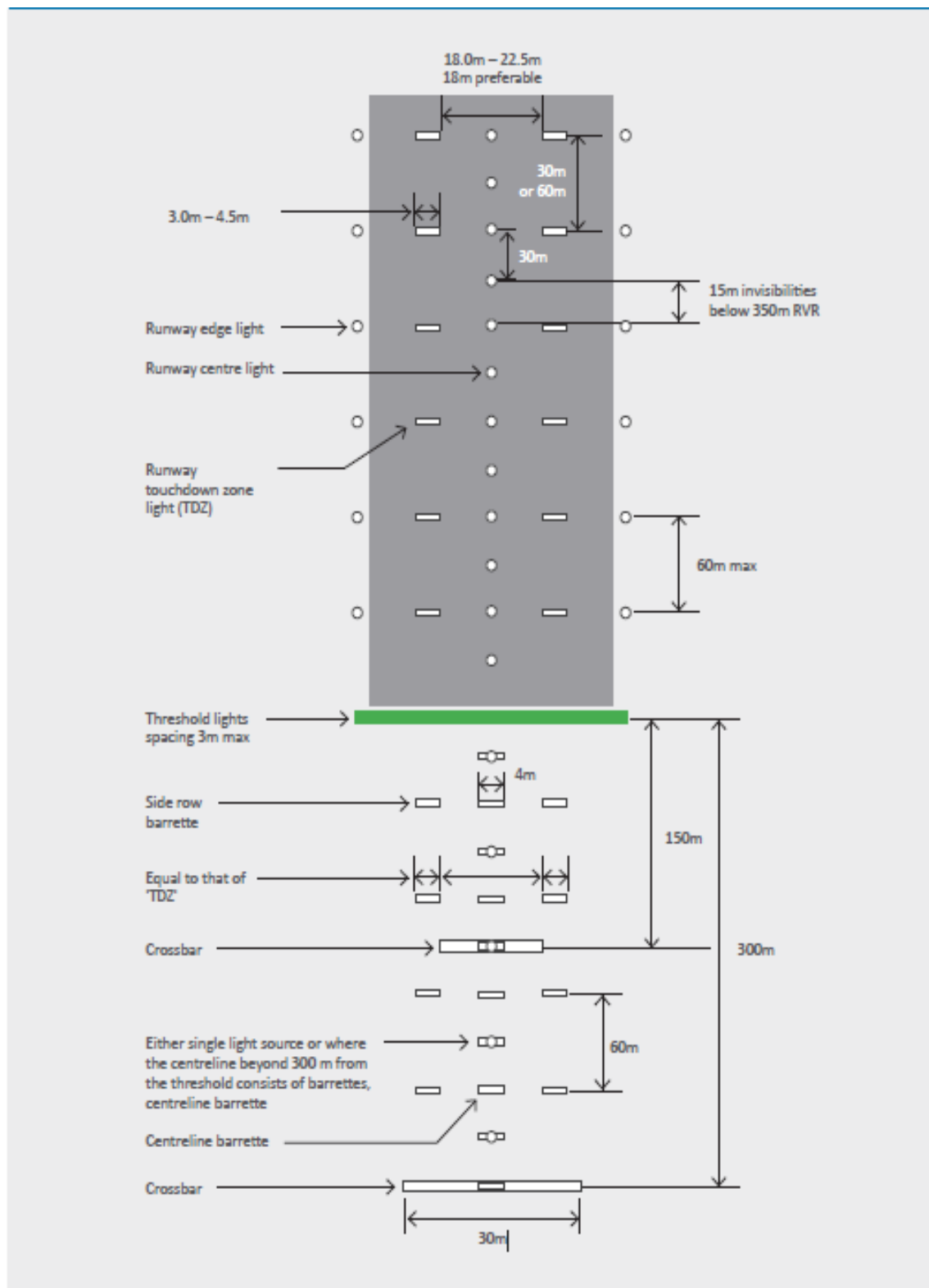
Figure 5-9. Inner typical 300m of CAT II & CAT III
