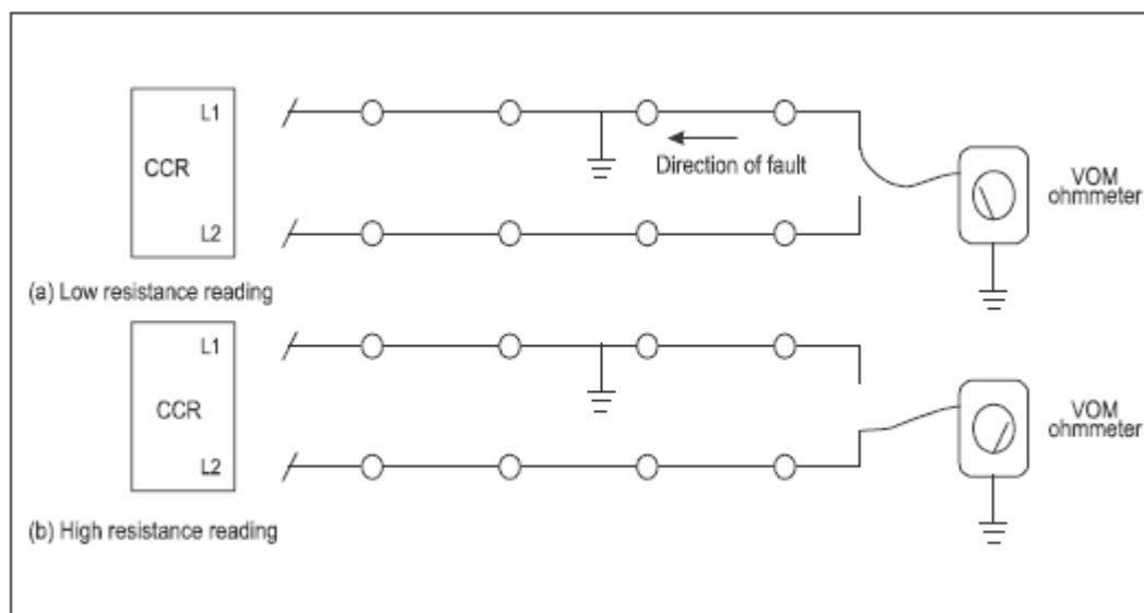
Figure 6-3 a, b. Locating Ground Faults with the VOM
