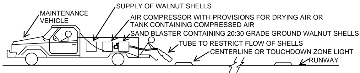
Figure 5-3. Cleaning Runway Centerline and Touchdown Zone Lights.
