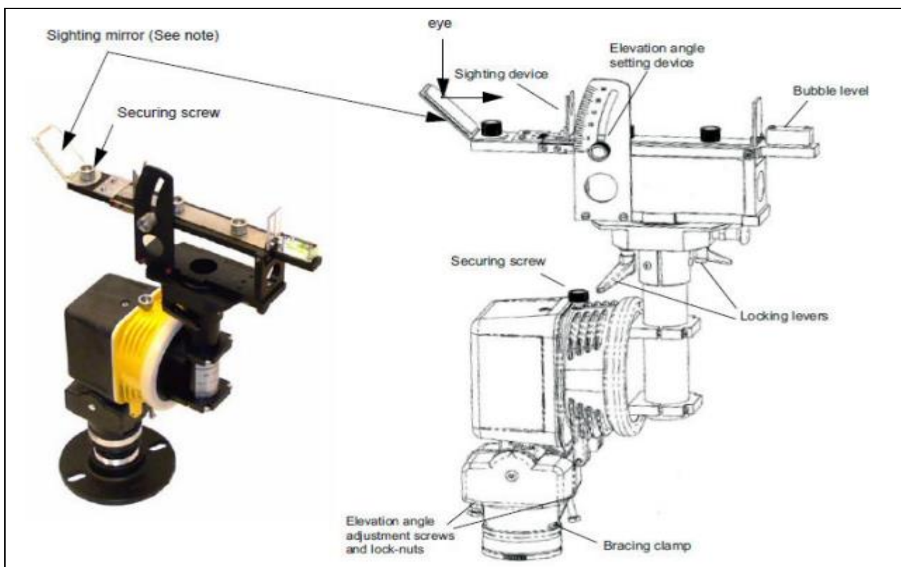
Figure 5-6. Installation of RTIL Aiming unit
