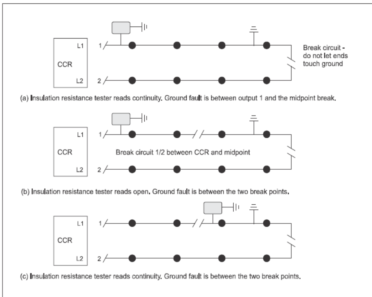
Figure 6-4. Alternative Method of Finding Ground Fault Using VOM or Insulation Resistance Tester
