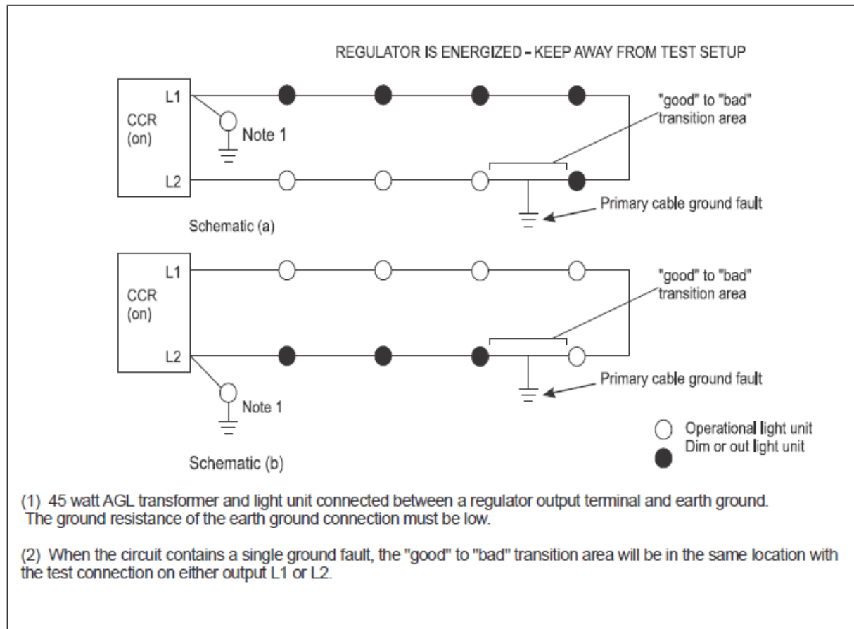
Figure 6-8a, b. Intentional Ground Test
