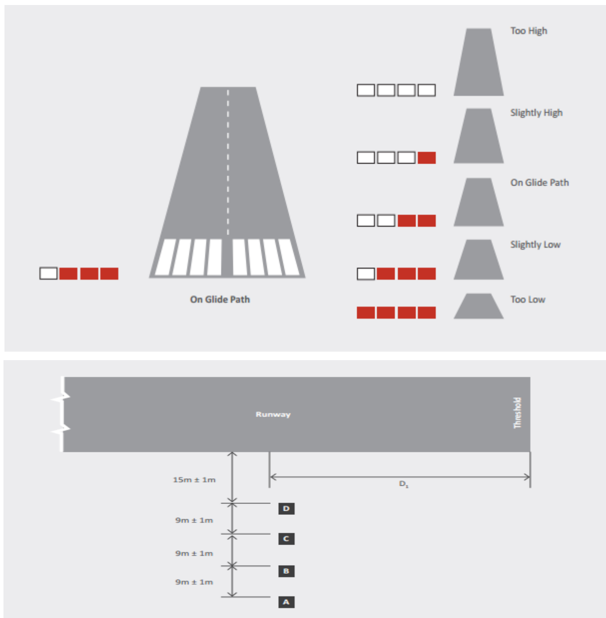
Figure 5-4. PAPI Configuration.
