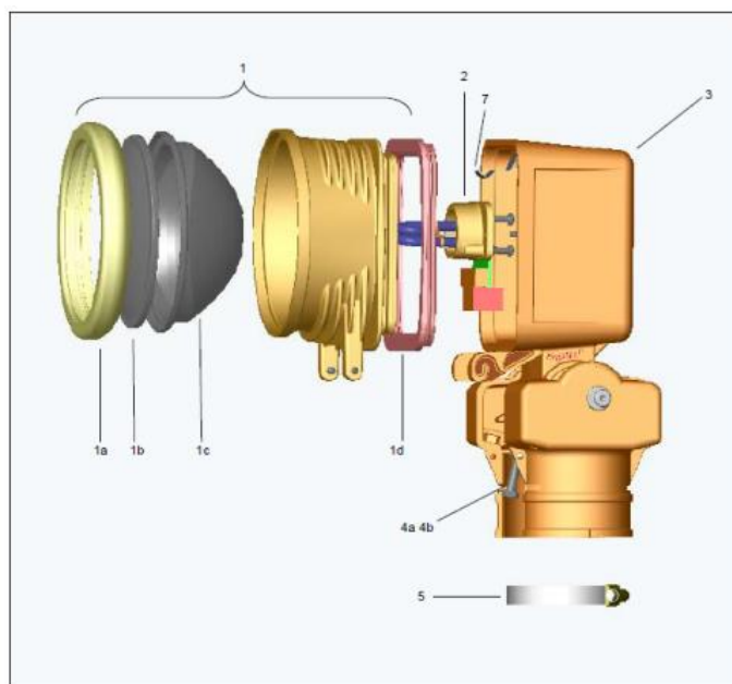
Figure 5-5. RTIL fixture.
