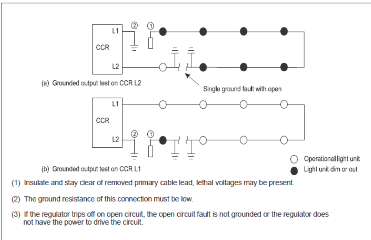
Figure 6-10a, b. Grounded Output Test
