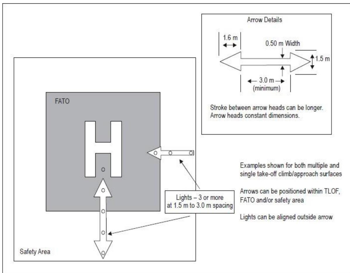
Figure 5-9. Flight path alignment guidance markings and lights
