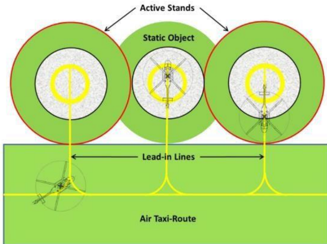
Figure 3-8. Turning stands designed for hover turns (with air taxi-routes) / non-simultaneous use – outer stands active
