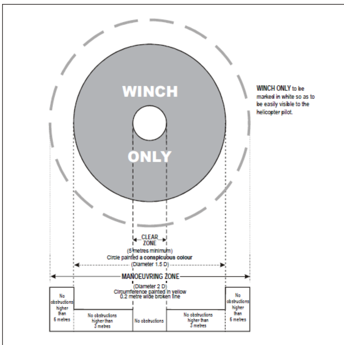
Figure 4-12. Winching area of a ship
