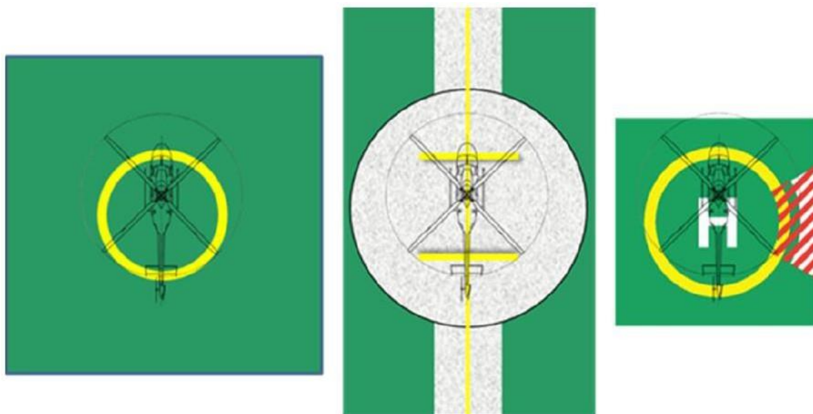
Figure 5-7. (Left) multidirectional TDPC with no limitations. (Centre) unidirectional marking shoulder line with associated centreline. (Right) multidirectional TDPC with prohibited landing sector marking
