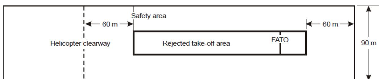
Figure A1-1. Safety area for instrument FATO
