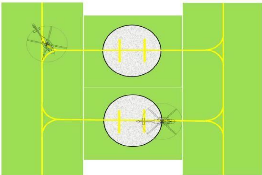
Figure 3-7. Air taxi-through stands (with air taxi-route) simultaneous use
