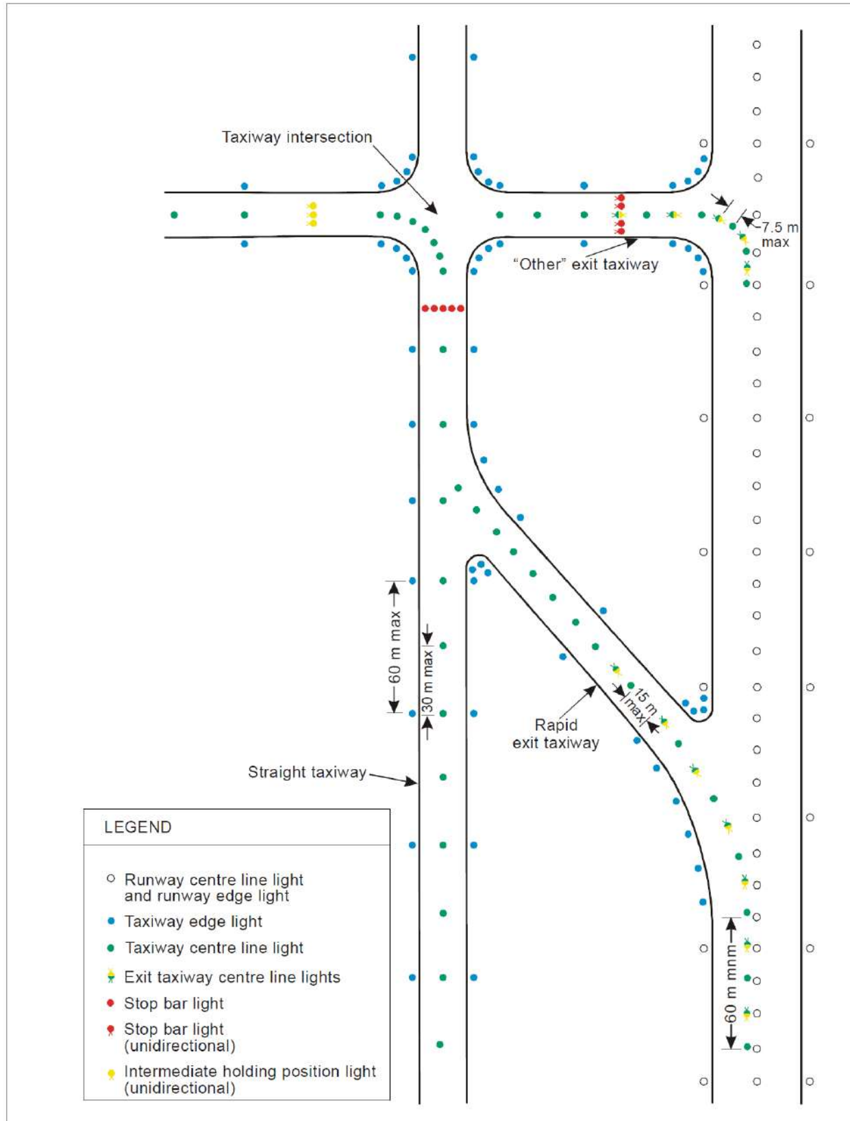
Figure 5-24. Taxiway Lighting
