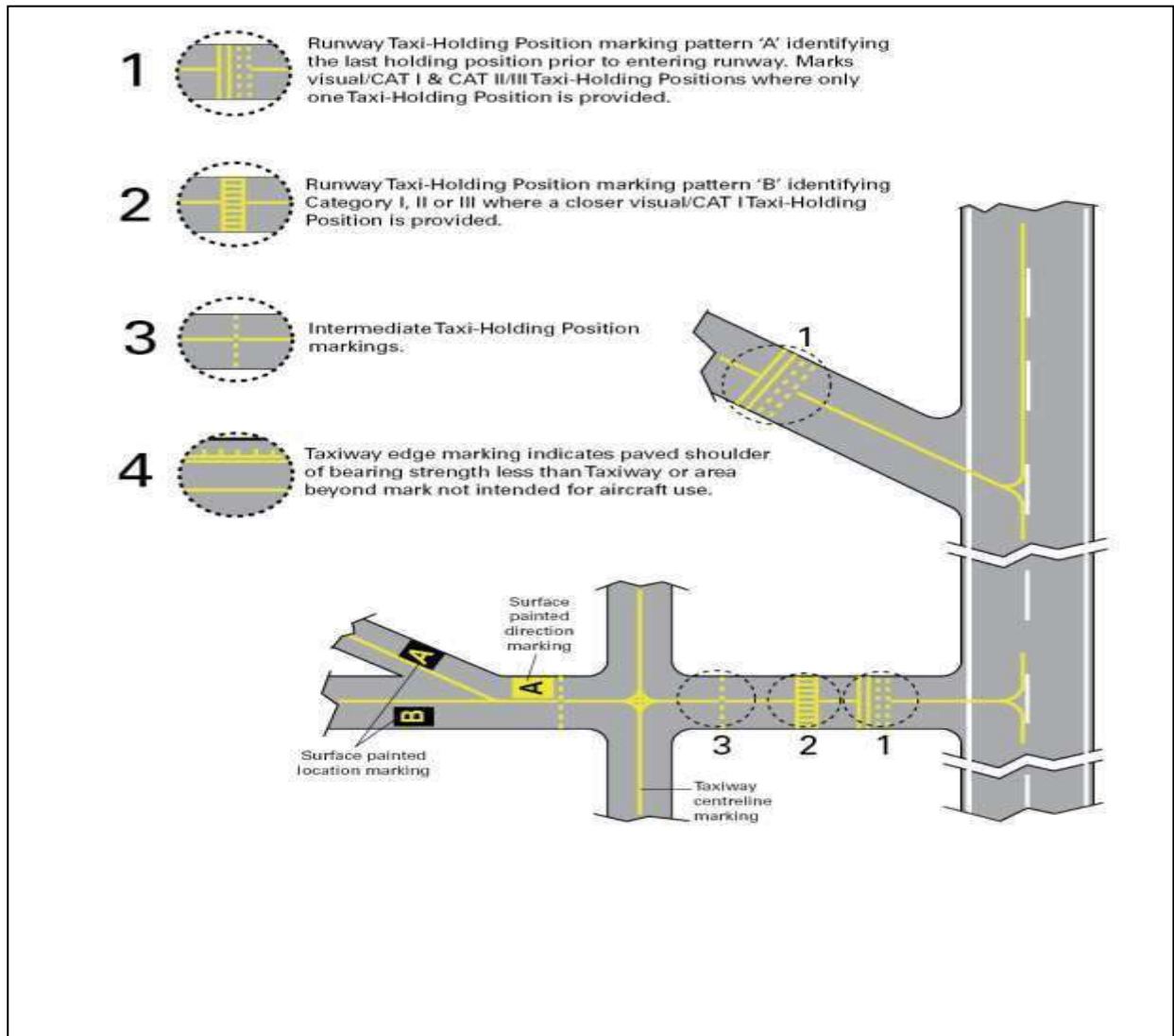
Figure 5-6 Taxiway markings
