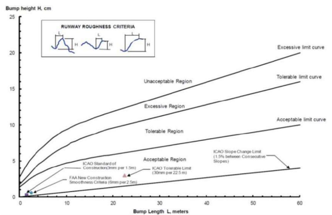
Figure A-3. Comparison of roughness criteria
