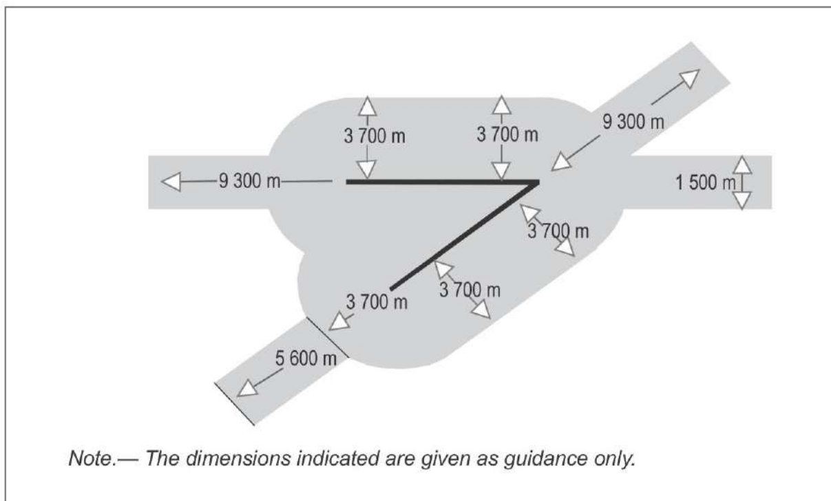
Figure 5-12. Multiple runway laser-beam free flight zone
