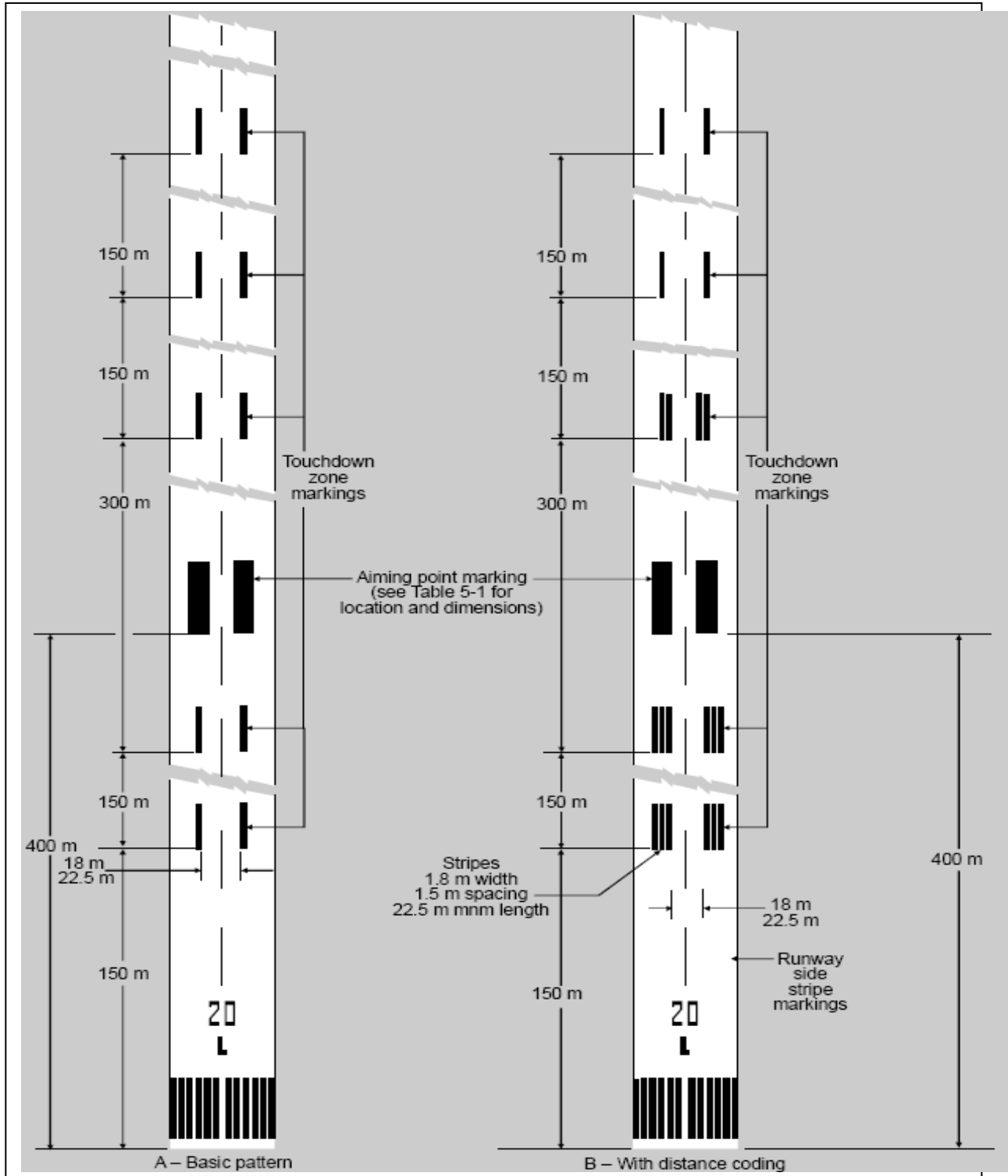
Figure 5-5 Aiming point and touchdown zone markings (Illustrated for a runway with a length of 2400m or more)
