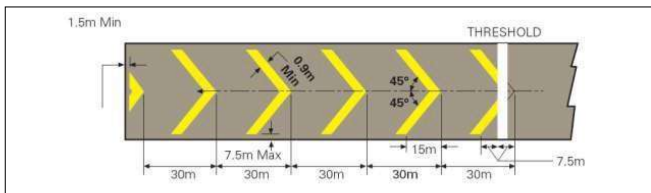
Figure 7-4. Pre-threshold marking
