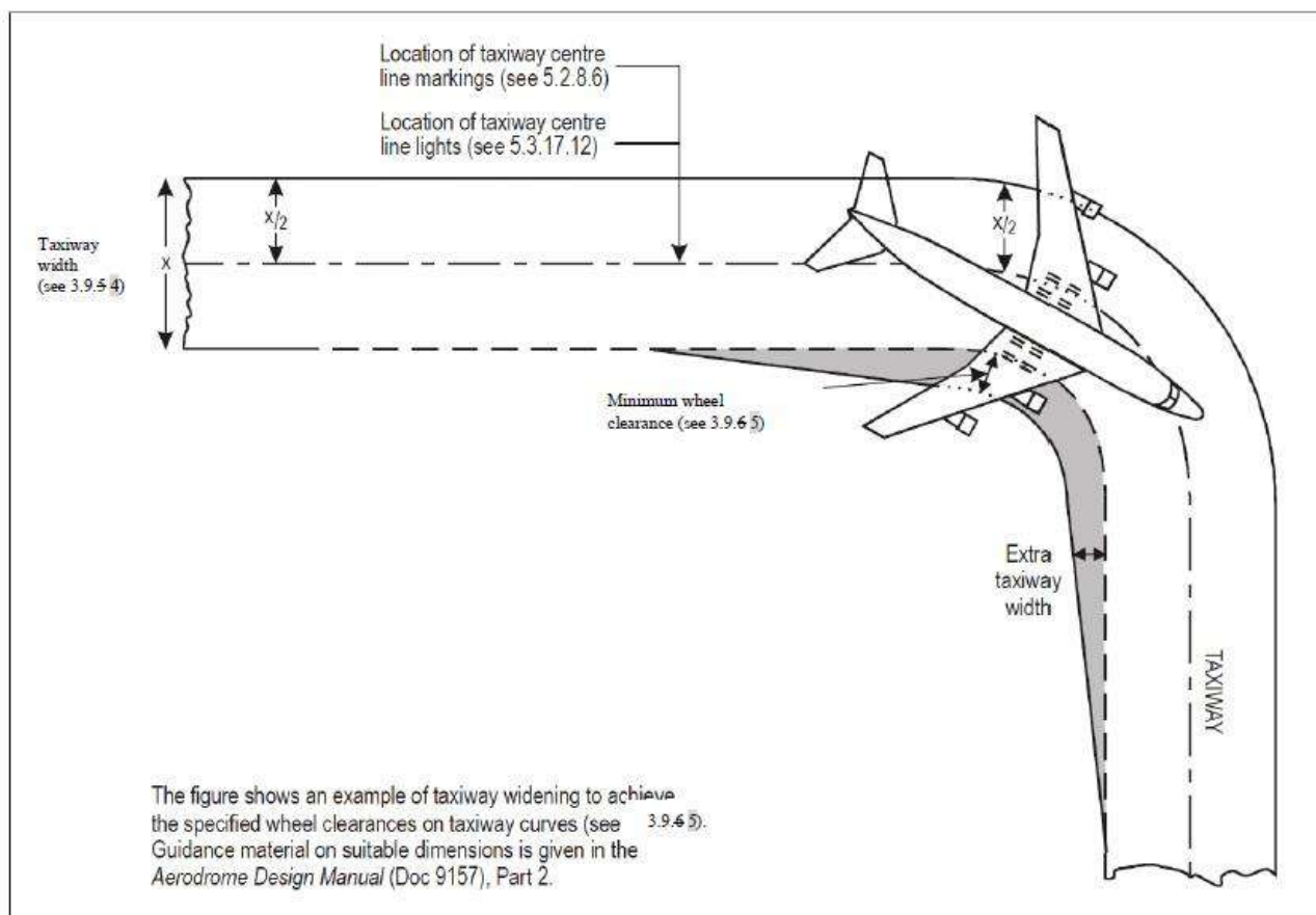
Figure 3.2. Taxiway curve
