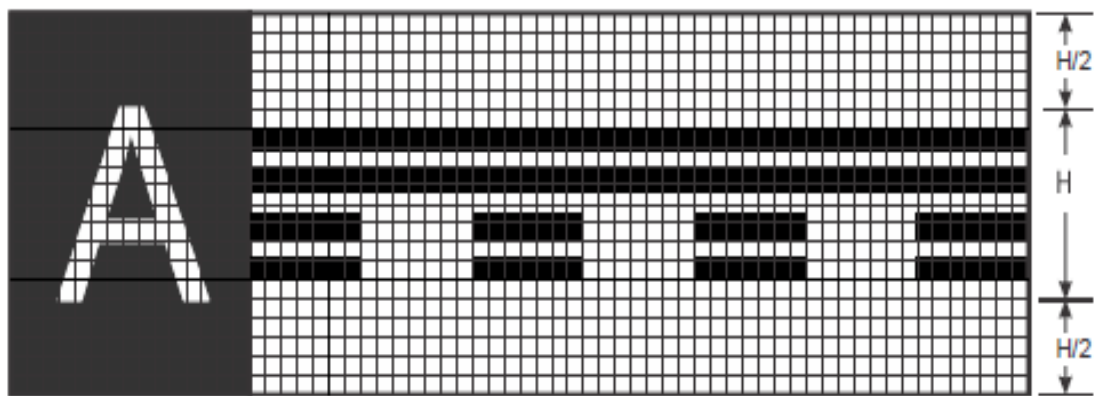
Runway vacated sign (with typical location sign)
