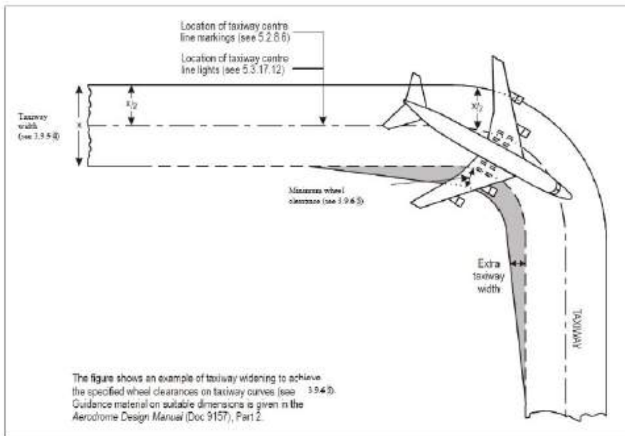
Figure 3.2. Taxiway curve
