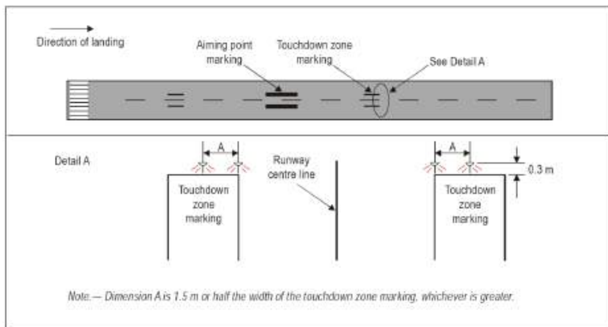
Figure 5-22. Simple Touchdown Zone Lighting
