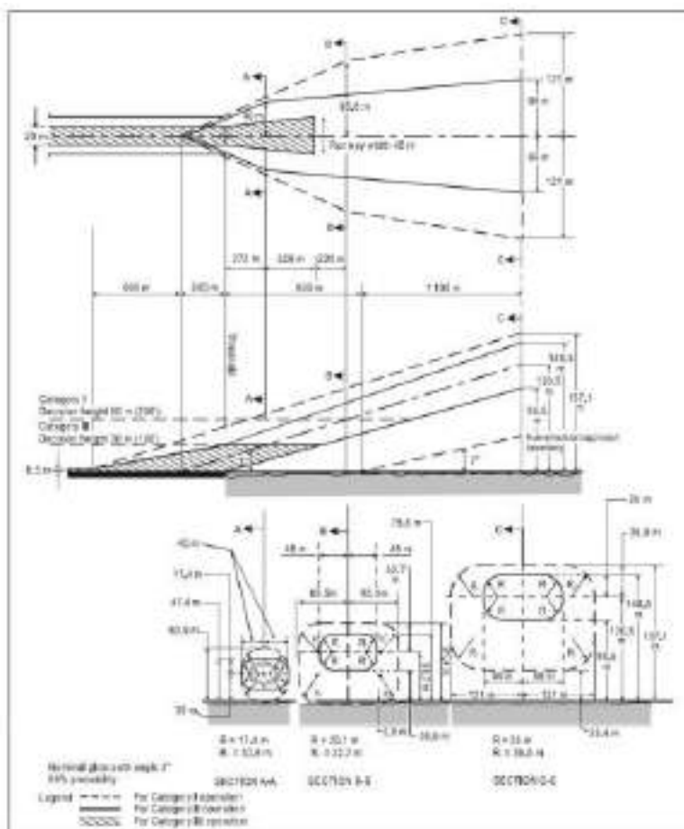
Figure A-6. Flight path envelopes to be used for lighting design for categories I, II and III operations
