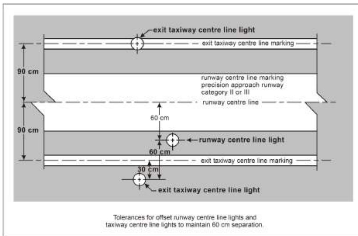
Figure 5-25. Offset Runway and Taxiway CenterLine Lights
