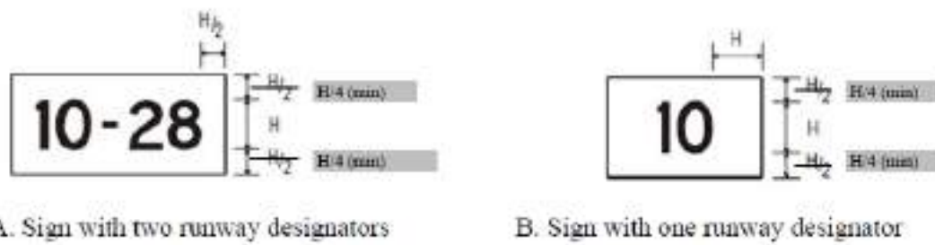
Figure A4-4. Sign dimensions
