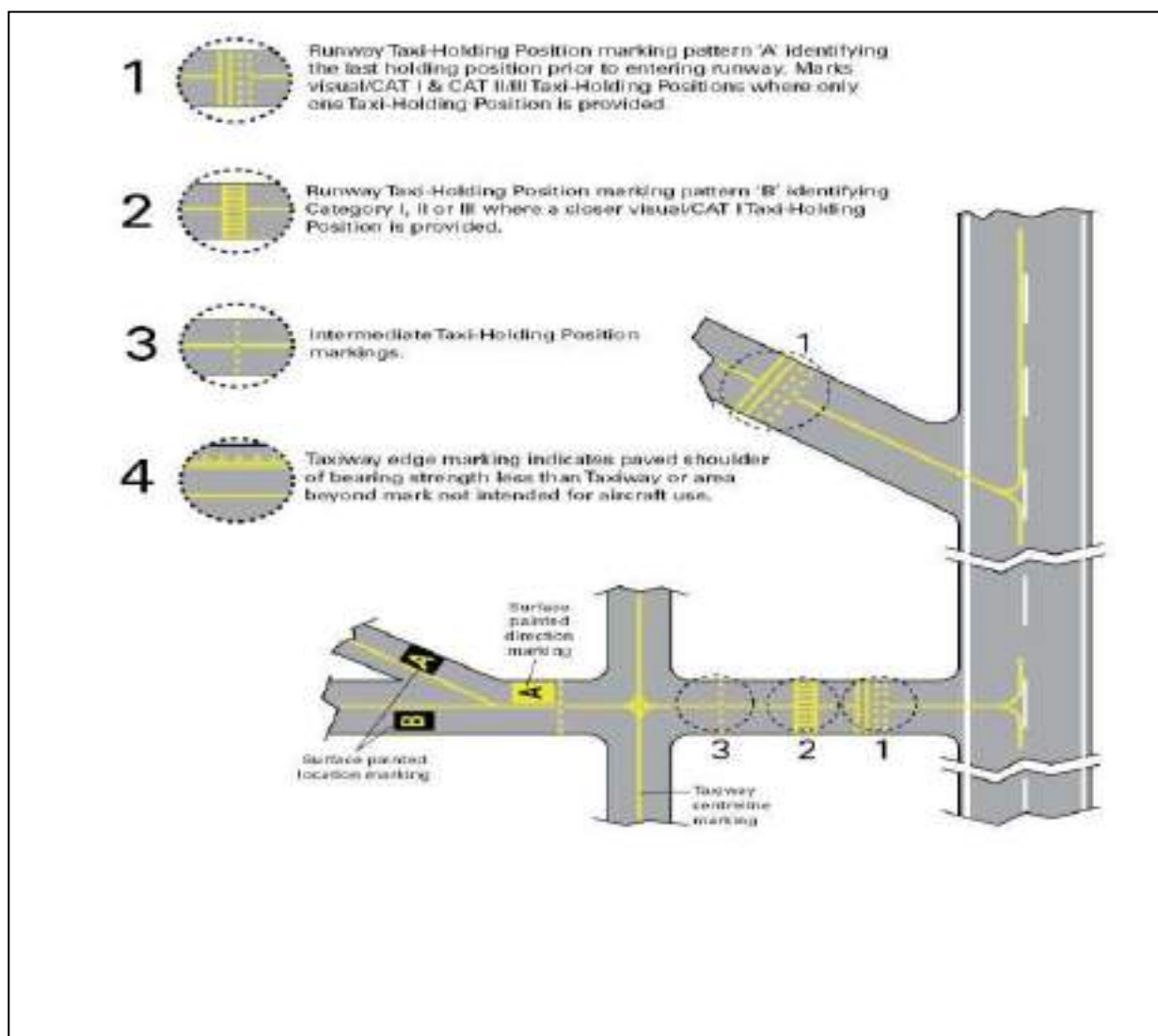
Figure 5-6 Taxiway markings
