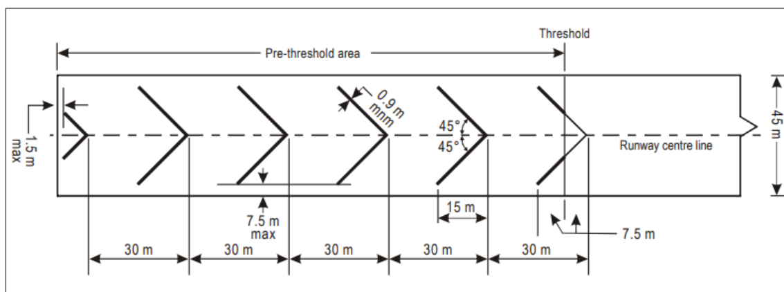
Figure 7-4. Pre-threshold marking
