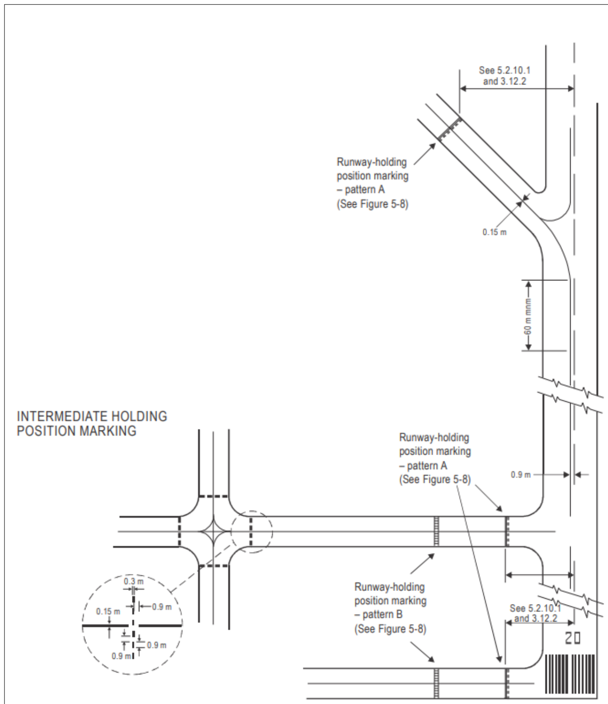
Figure 5-6 Taxiway markings
