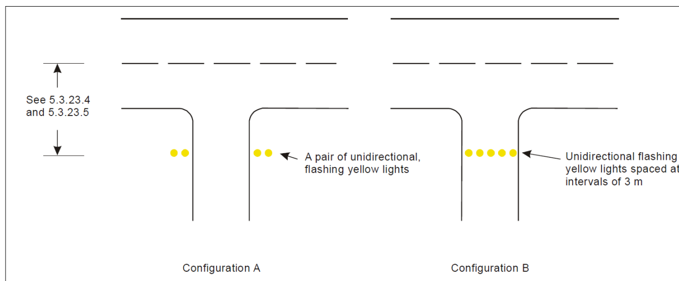
Figure 5-26. Runway Guard Light
