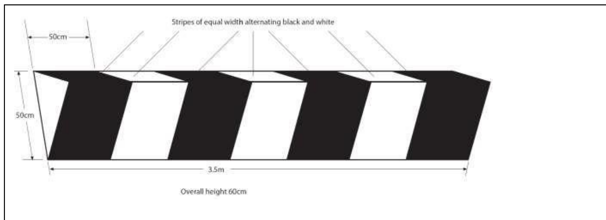
Figure 7-2. Temporary threshold marker board
