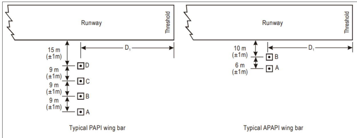
Figure 5-17 Sitting of PAPI and APAPI
