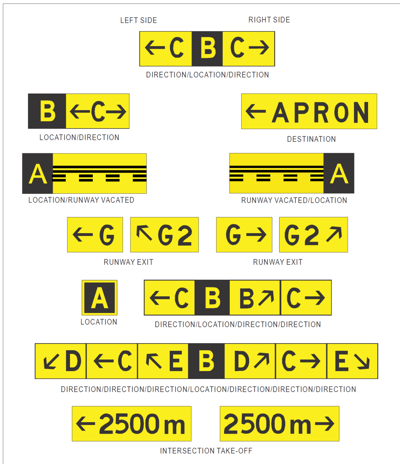
Figure 5-28. Information signs
