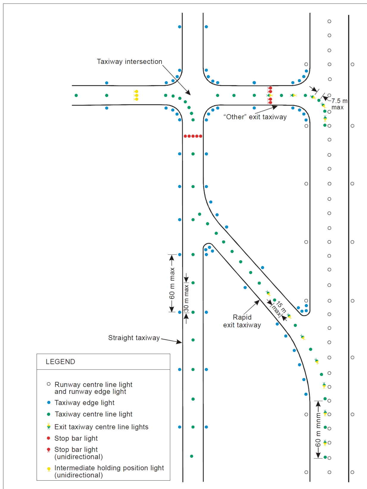
Figure 5-24. Taxiway Lighting
