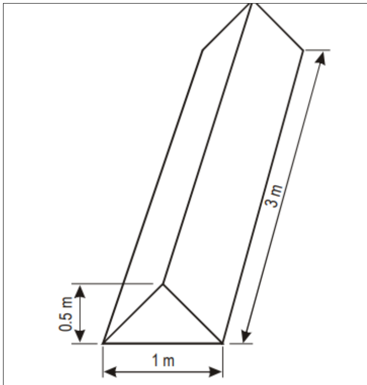
Figure 5-32. Boundary Markers
