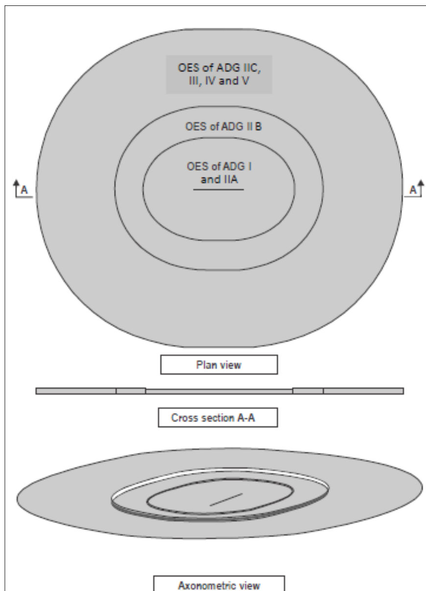
Figure 4-4. Horizontal surface
