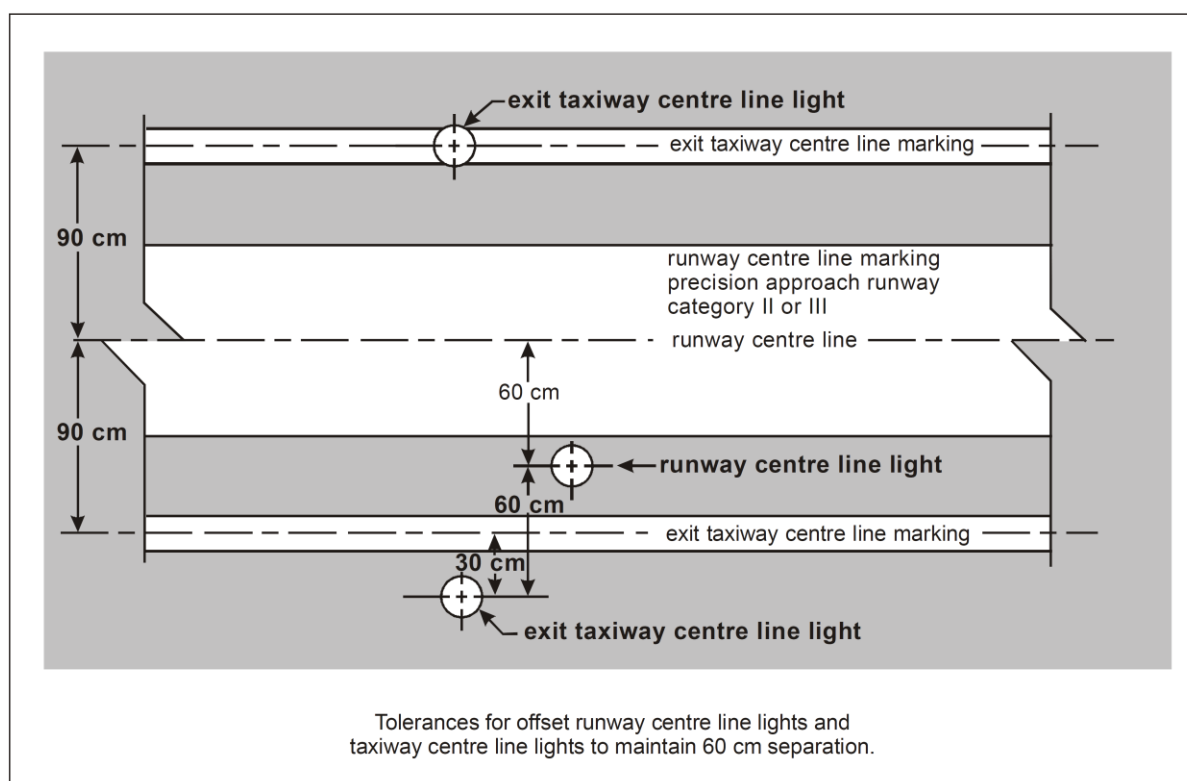
Figure 5-25. Offset runway and taxiway centre line lights
