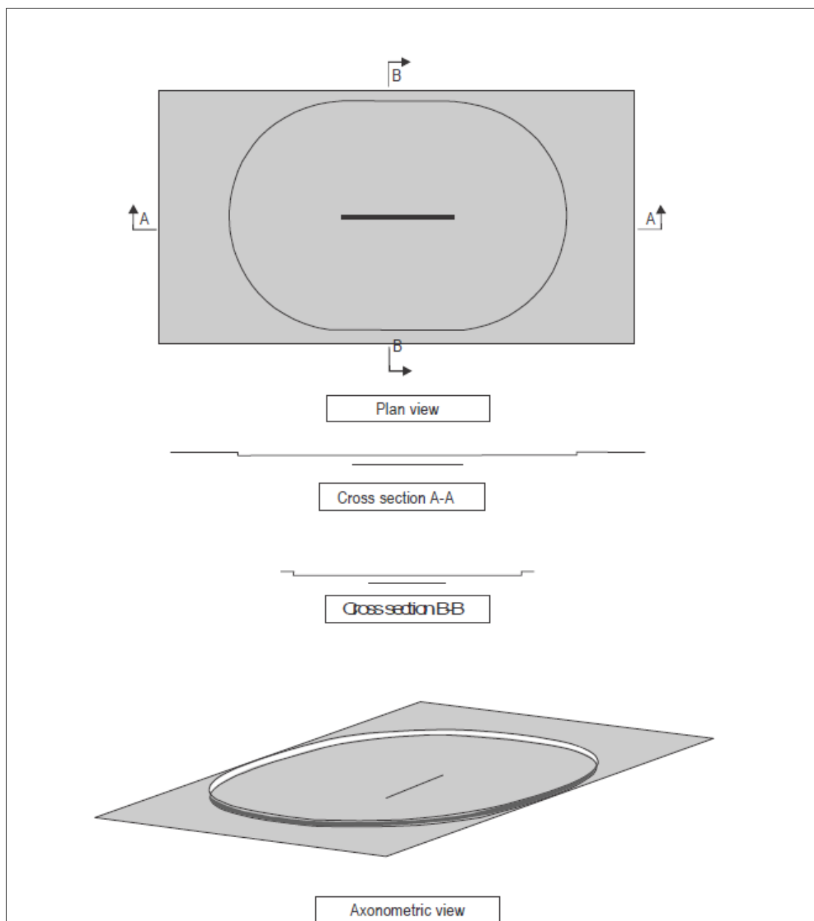
Figure 4-5. Surface for straight-in instrument approaches
