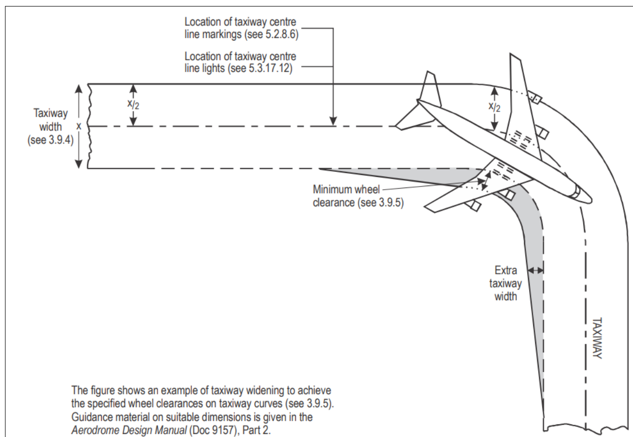
Figure 3-2. Taxiway curve
