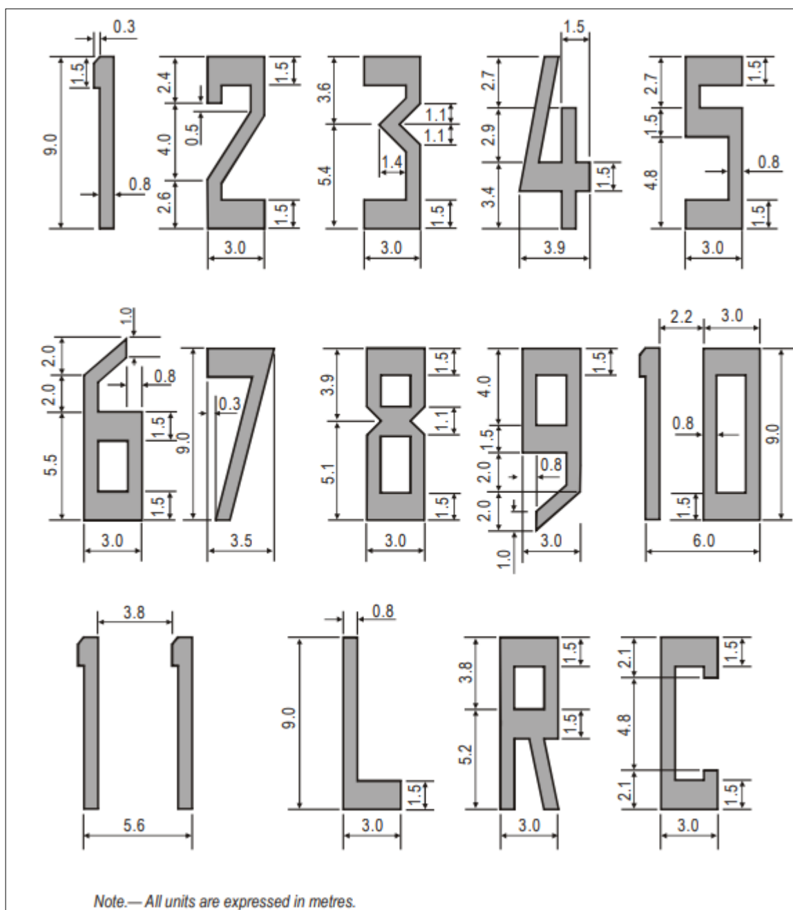
Figure 5-3. Form and proportions of numbers and letters for runway designation markings
