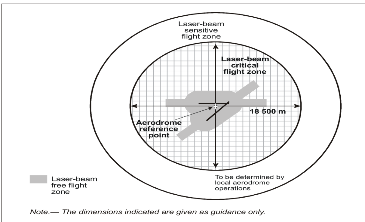
Figure 5-11. Protected Flight Zone
