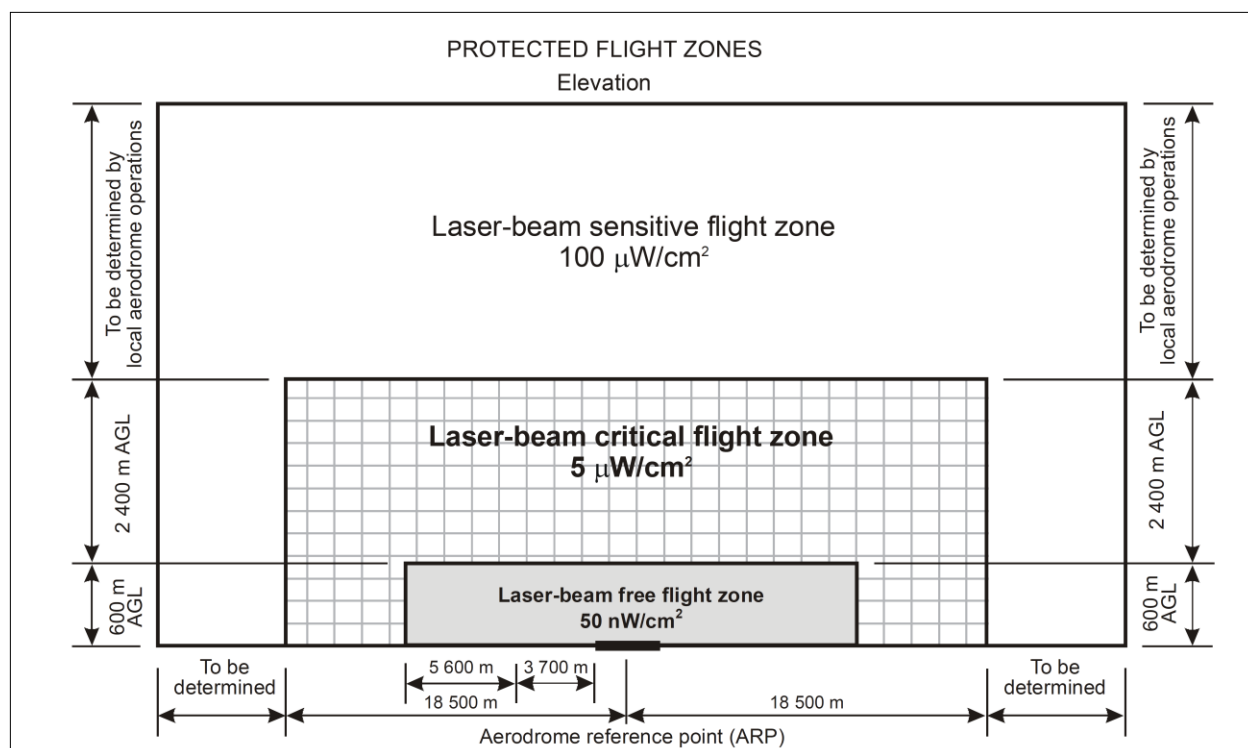
Figure 5-13. Protected flight zones with indication of maximum irradiance levels for visible laser beams
