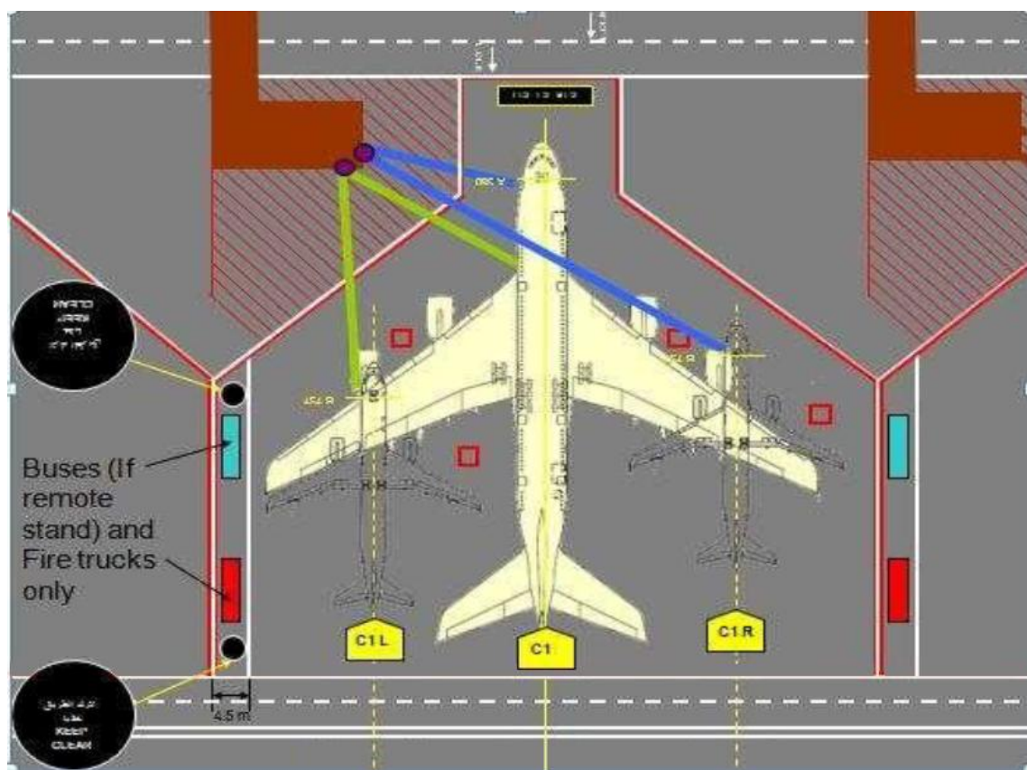
Apron safety lines marking
