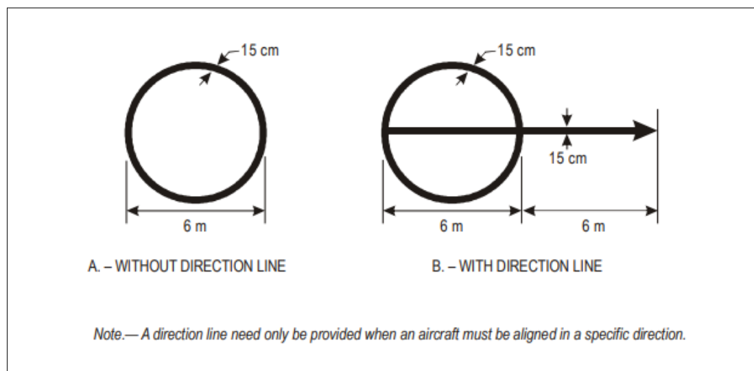
Figure 5-9. VOR aerodrome checkpoint marking
