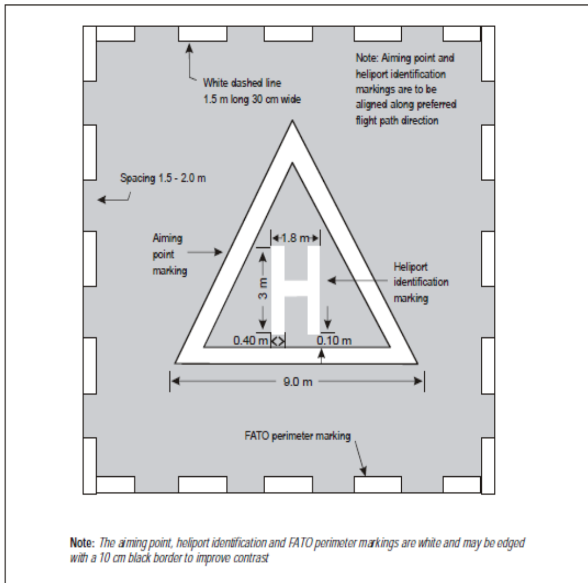
Figure 5-1. Combined heliport identification, aiming point and FATO perimeter marking
