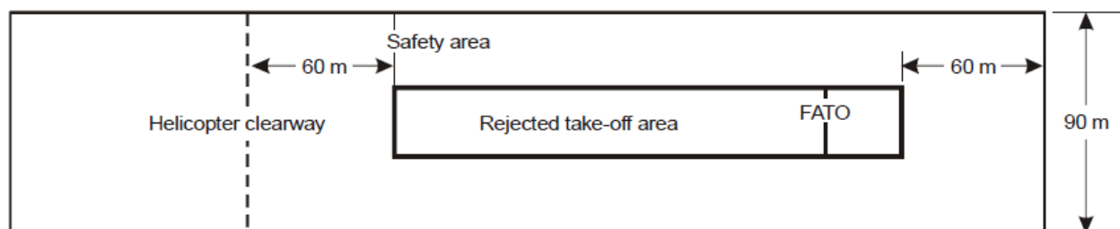
Figure A1-1. Safety area for instrument FATO
