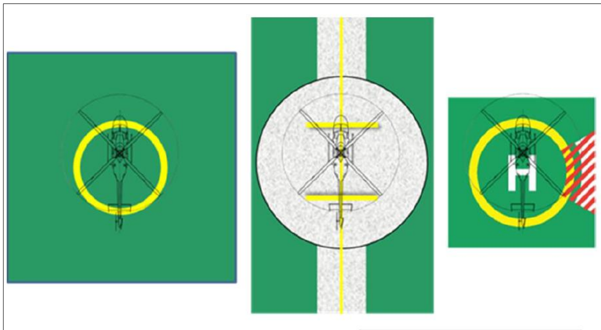
Figure 5-8. Multidirectional TDPC with no limitations (Left) Unidirectional marking shoulder line with associated centreline (Centre) Multidirectional TDPC with prohibited landing sector marking (Right)
