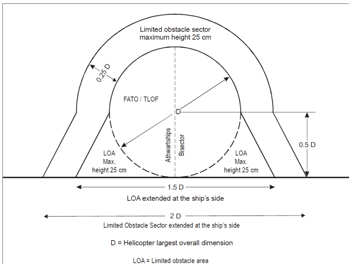
Figure 4-6. Ships-side non-purpose-built heliport obstacle limitation sectors and surfaces
