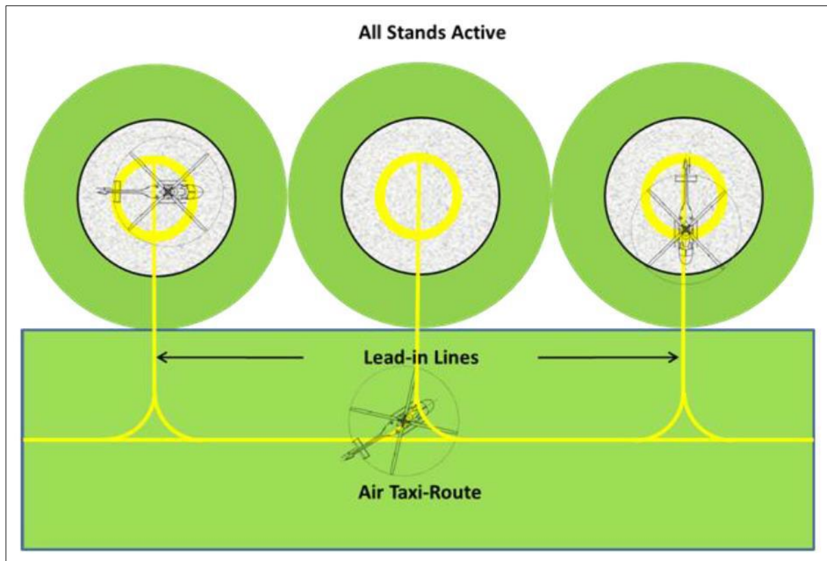
Figure 3-5. Turning stands (with air taxi-routes) simultaneous use
