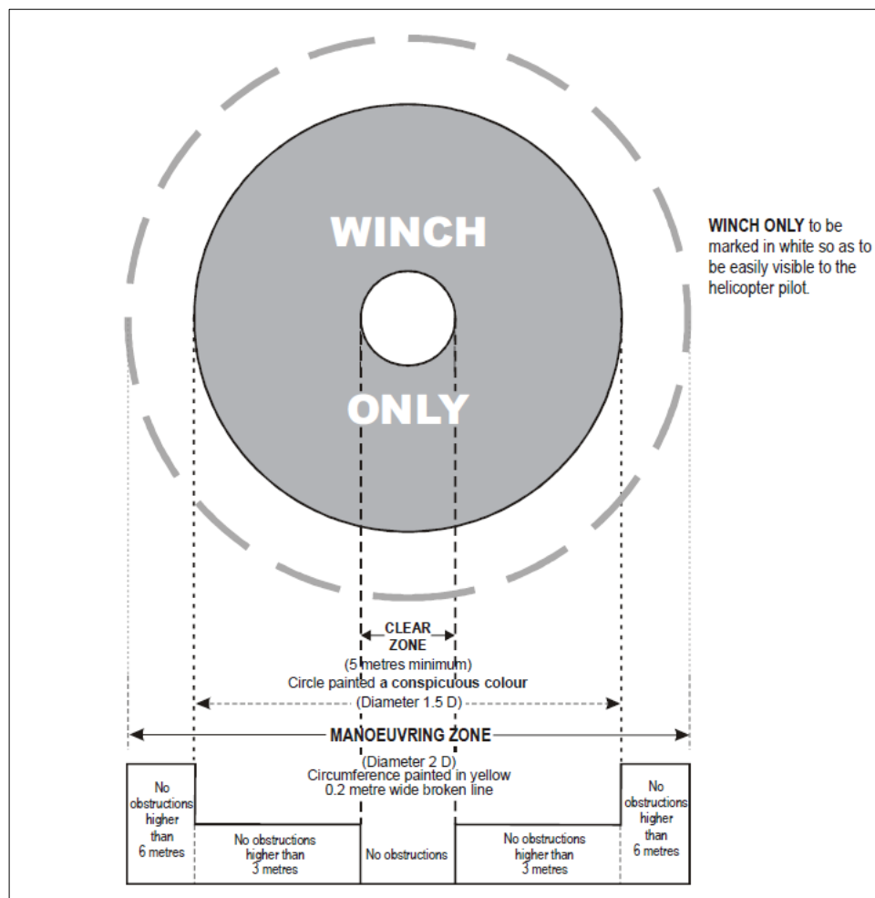
Figure 4-12. Winching area of a ship
