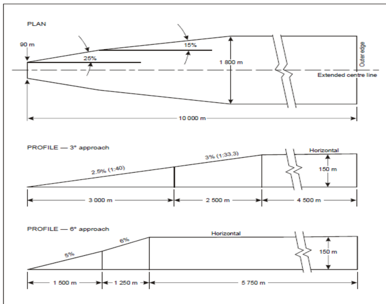
Figure A1-3. Approach surface for precision approach FATO
