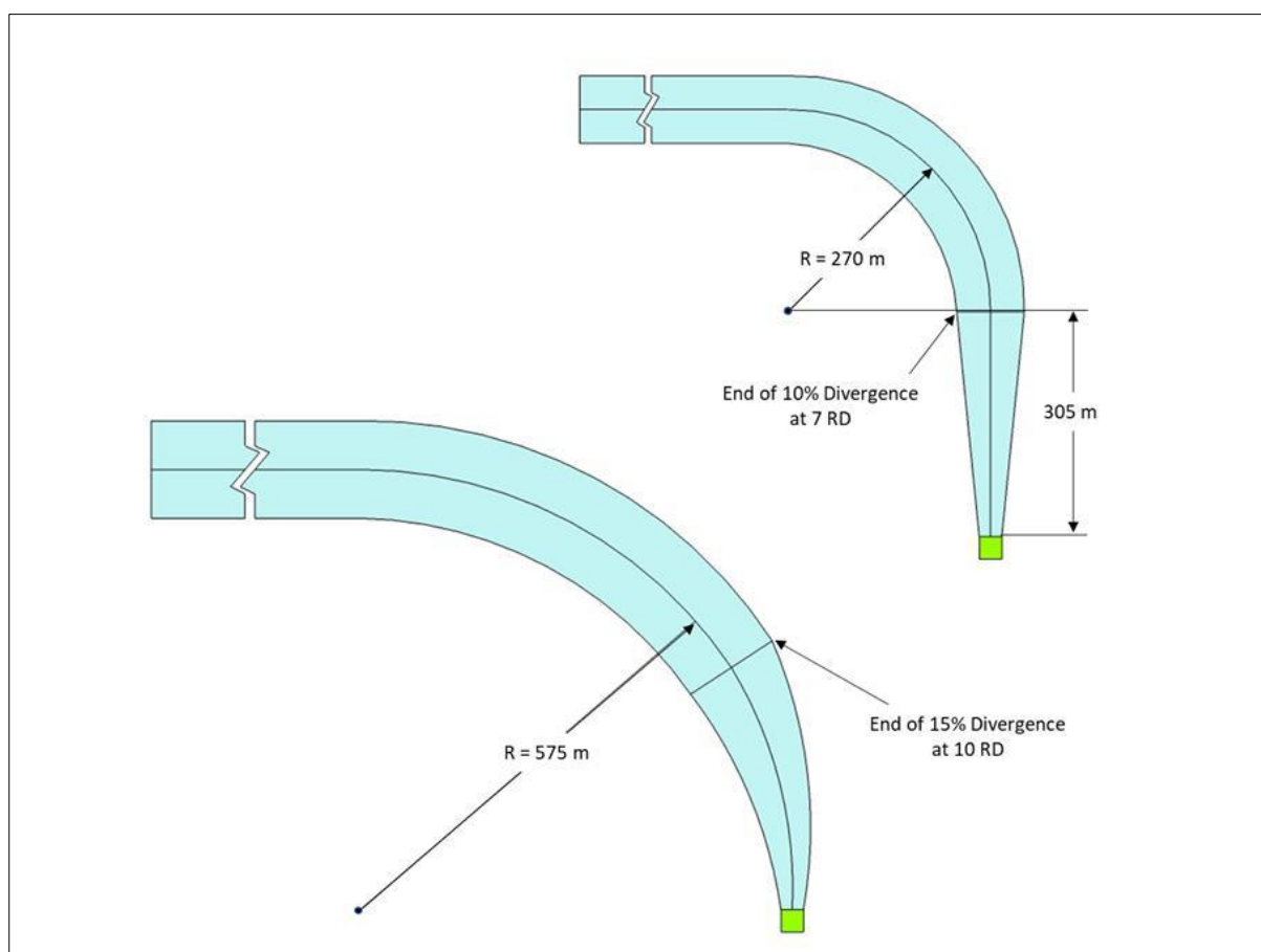
Figure 4.1. Curved approach and take-off climb surface for all FATOs
