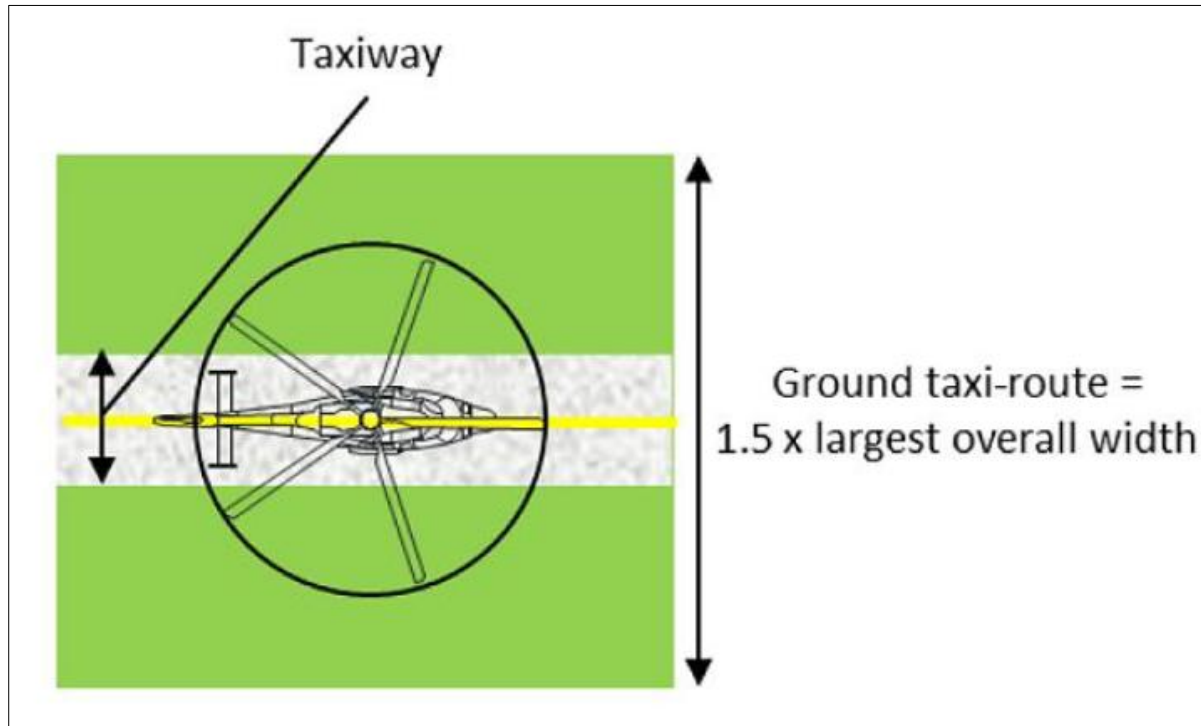
Figure 3-3. Helicopter taxiway/ground taxi-route
