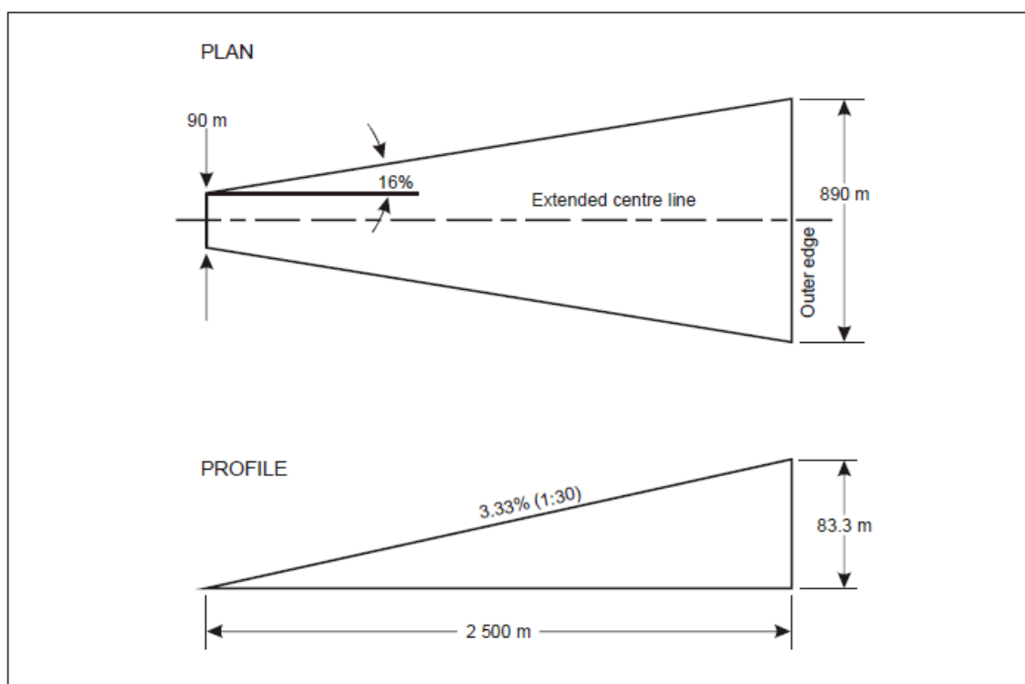
Figure A1-4. Approach surface for non-precision approach FATO
