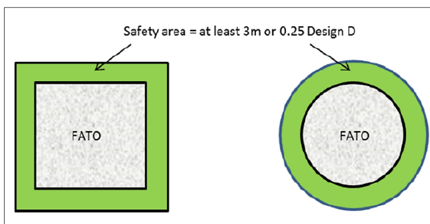
Figure 3-1. FATO and associated safety area
