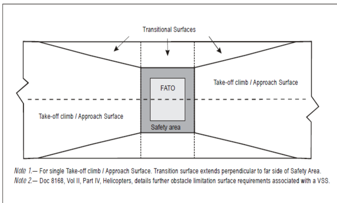
Figure A1-5. Transitional surfaces for an instrument FATO with a non-precision and/or precision approach
