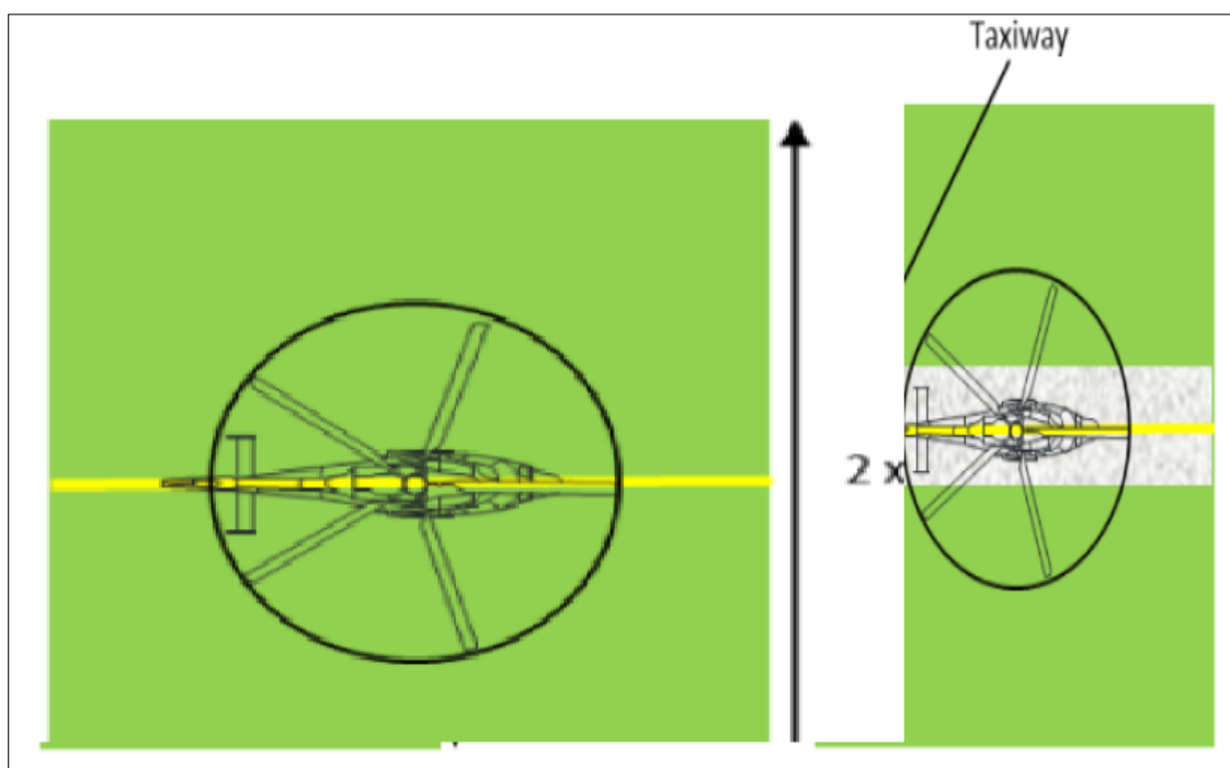
Figure 3-3. Helicopter air taxi-route and combined air taxi-route/taxiway
