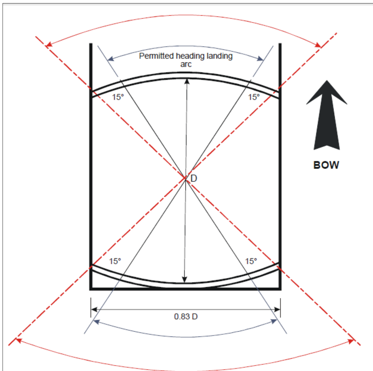
Figure 3-10. Shipboard permitted landing headings for limited heading operations
