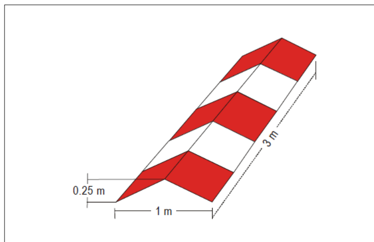
Figure 5-6. Runway-type FATO edge marker
