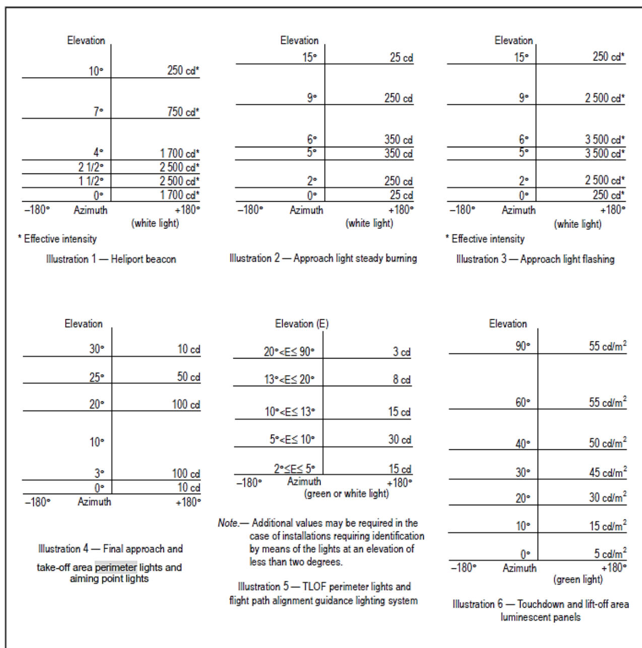
Figure 5-12. Isocandela diagrams
