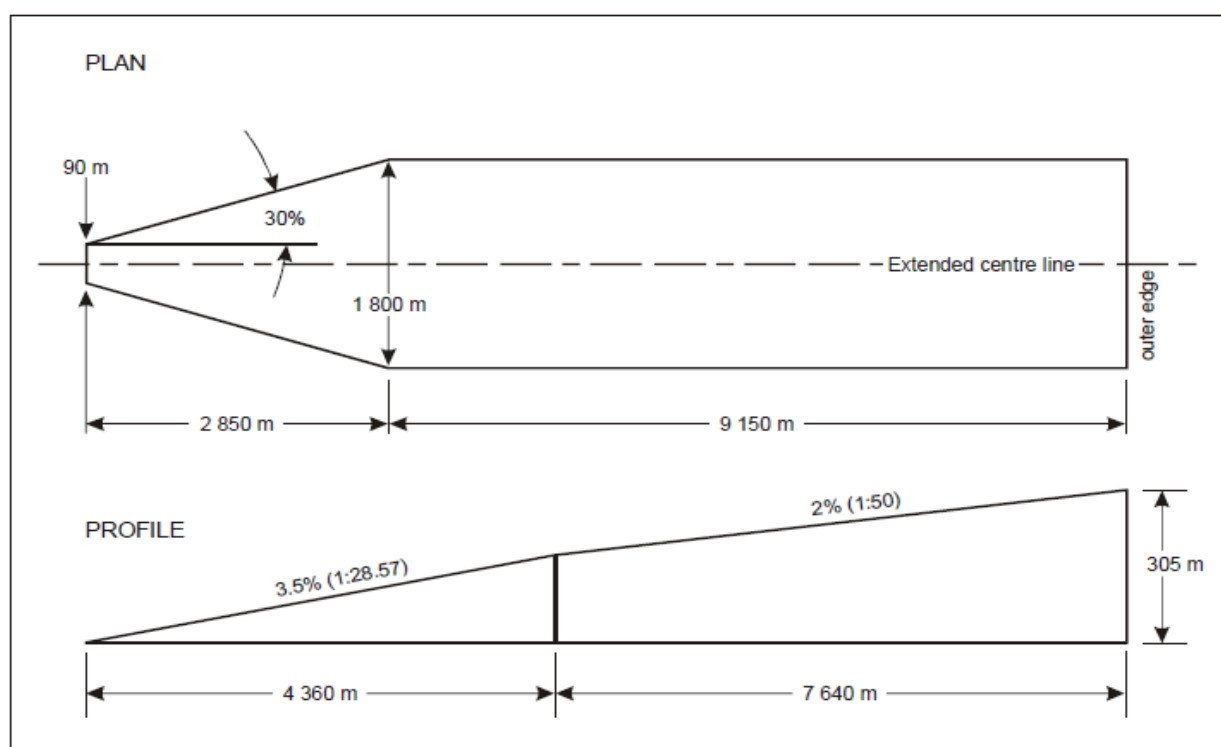
Figure A1-2. Take-off climb surface for instrument FATO
