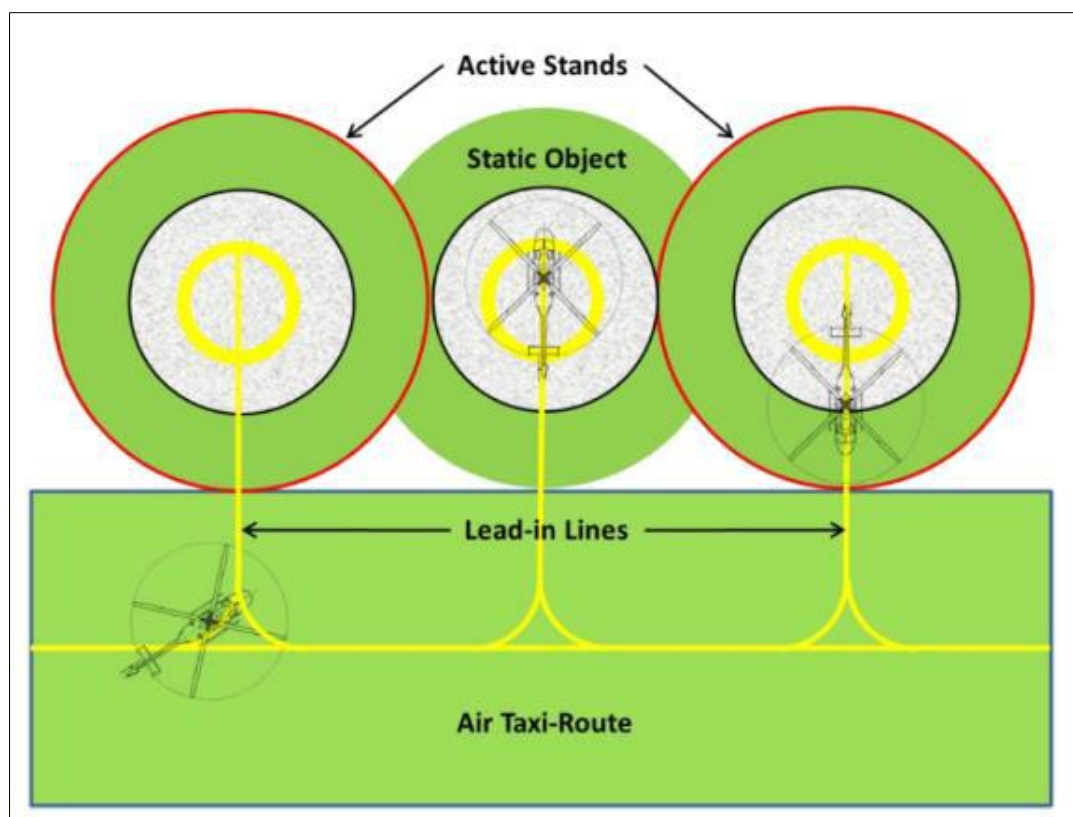
Figure 3-8. Turning stands designed for hover turns (with air taxi-routes) / non-simultaneous use – outer stands active
