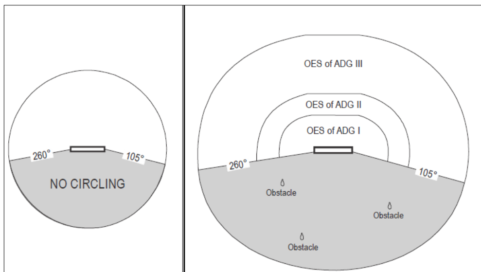
Figure 10-2. Modifying horizontal OES on a non-circling area
