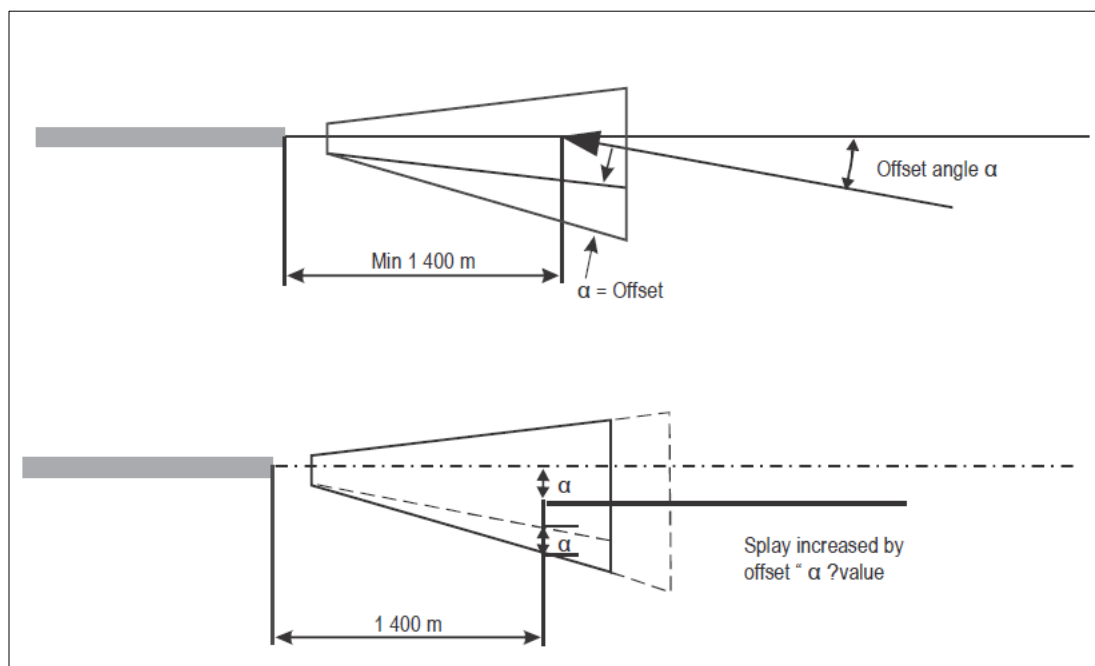
Figure 10-1. Plan view visual segment surface offset final approach with runway centre line crossing
